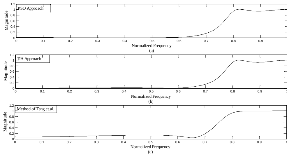
Fig. 3 Magnitude responses of HP filter using the PSO method and the methods given in [12] and [4], respectively.
