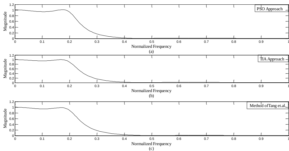
Fig. 2 Magnitude responses of LP filter using the PSO method and the methods given in [12] and [4], respectively.
