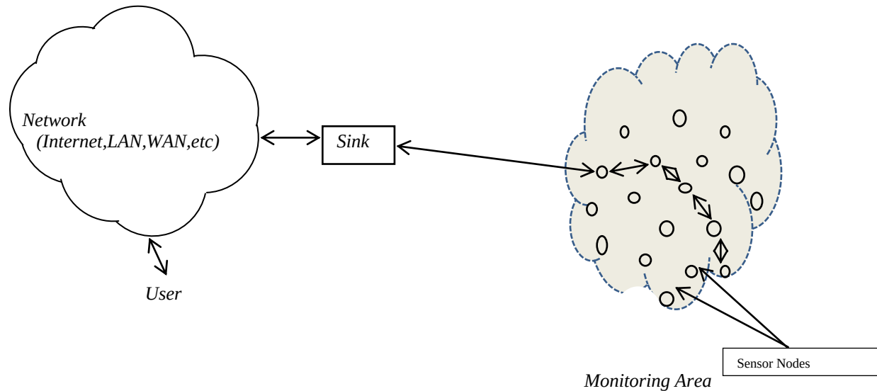
Figure 1: Sensors arrangement in a WSN. Nodes utilizing multi-hop communication and end user access the data through a network
