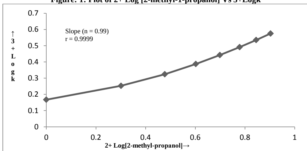
Figure: 1: Plot of 2 + \log [2\text{-methyl-1-propanol}] Vs 3 + \log k
