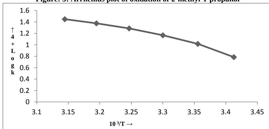
Figure 3: Arrhenius plot of oxidation of 2-methyl-1-propanol
