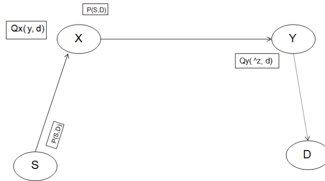
Figure 3. Q Routing Example
