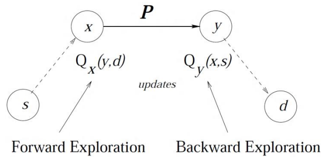
Figure 7. Dual reinforcement Q Routing(DRQ Routing).
