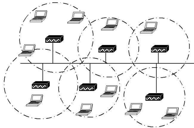
Figure 2. Example of Infrastructure Network
