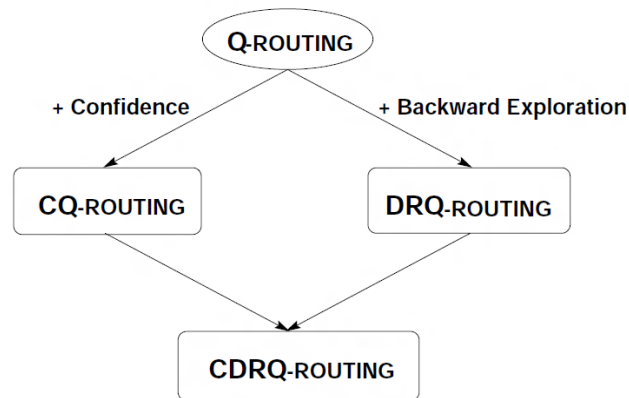
Figure 6. Optimzation of Q Routing.
