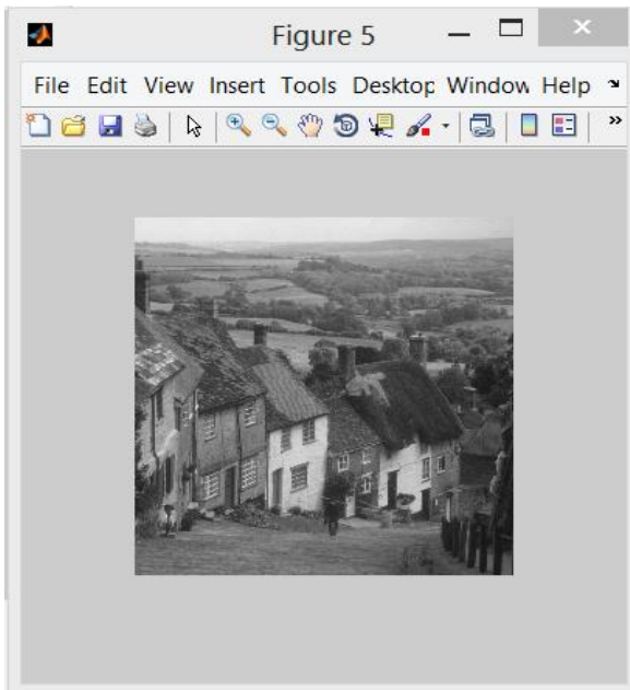
Fig.4: denoise image
