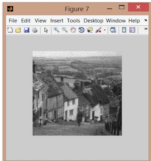
Fig. 5: noised image
