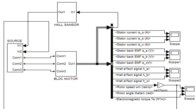
Fig 2. Simulink model of BLDC drive
