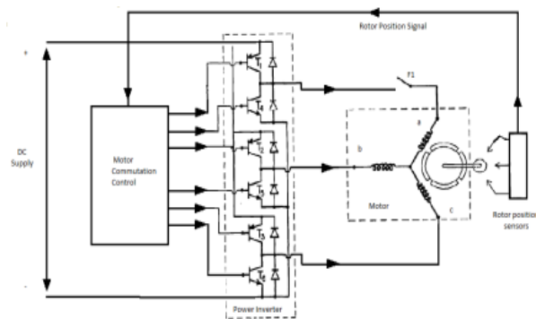
Fig 1. Complete Drive System
