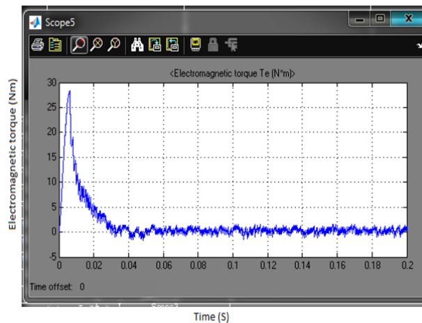
Fig 4. Electromagnetic torque (Nm) waveform for motor failure
