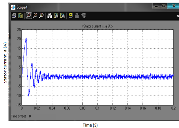
Fig 3. Stator current_a (A) waveform for motor failure
