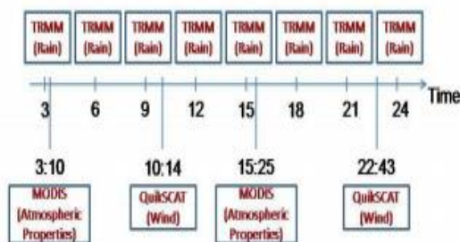
Figure 1. Data availability timeline from TRMM (3B42 data), QuikSCAT (L2B data) and Aqua (MODIS) on 18 Aug 2007 for Hurricane Dean
