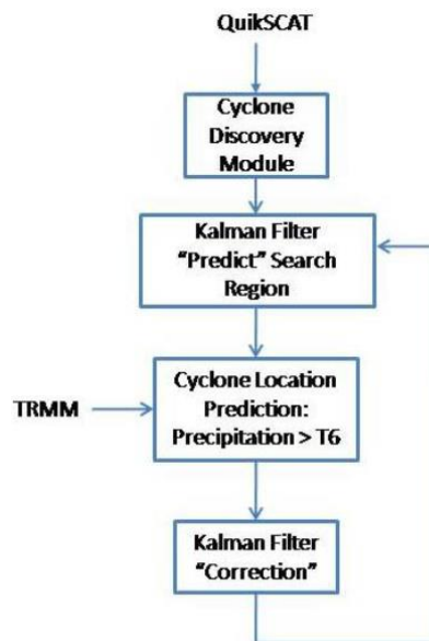
Figure 4. Knowledge sharing for Cyclone Tracking
