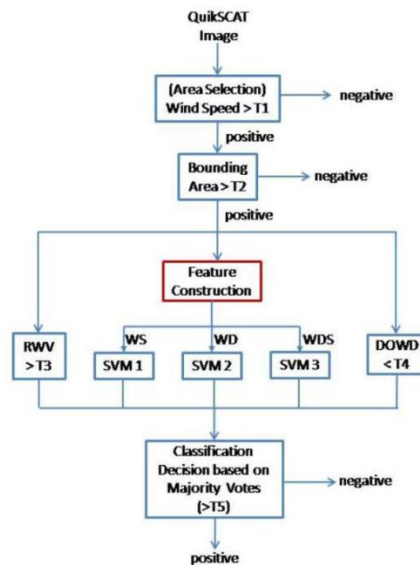
Figure 3. Ensemble Classifier (Cyclone Discovery Module)
