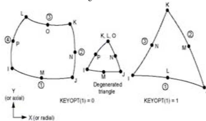
Figure 7: The geometry, node locations, and the coordinate system for element PLANE183 [17].
