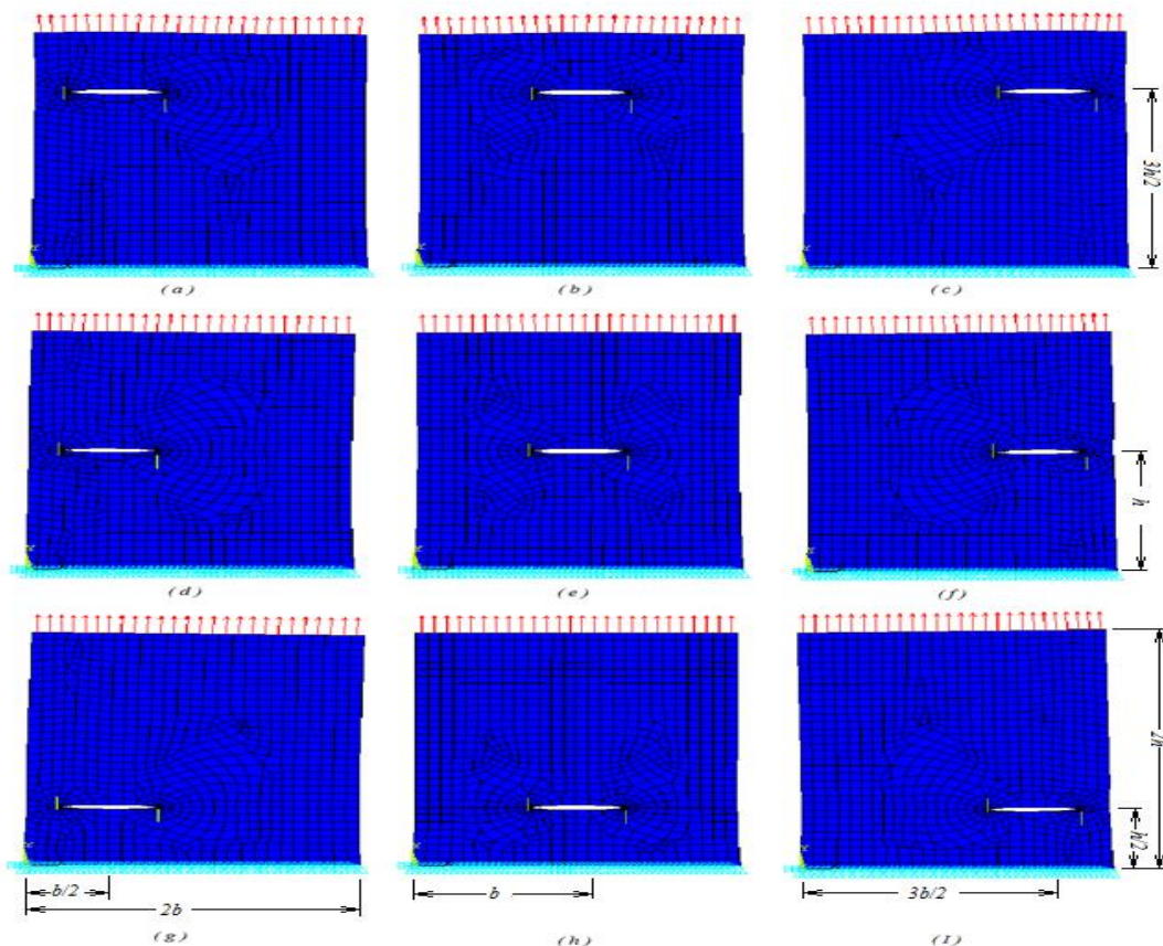
Figure 6: ANSYS models with mesh, elements and boundary conditions.
