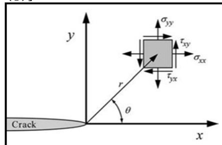
Figure 2: Definition of the coordinate axis ahead of a crack tip [13]
