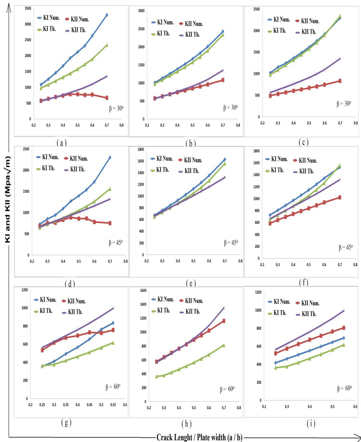
Figure 9: Variation of KI Num., KI Th., KII Num. and KII Th. with the variation of a/b for b, e and h model at \beta = 30, 45 and 60^\circ .
