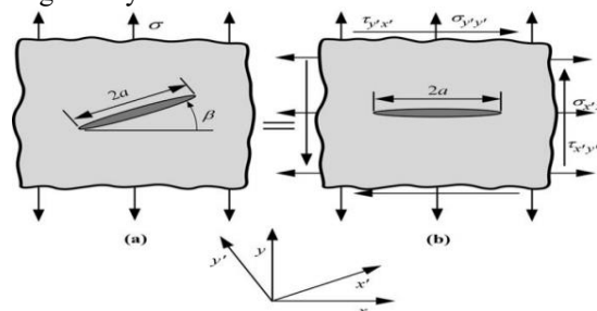
Figure 4: Through crack in an infinite plate for the general case where the principal stress is not perpendicular to the crack plane [13].
