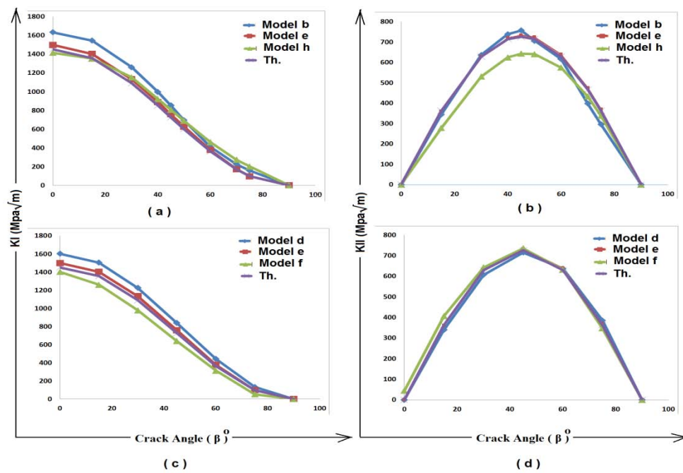
Figure 10: Variation of KI and KII with the crack angle: a and b) for model b, e, h and theoretical. c and d) for model d, e, f and theoretical.
