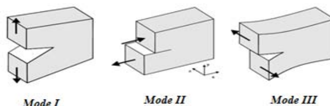
Figure 1: Three standard loading modes of a crack [12].
