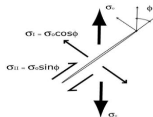
Figure 3: Crack subjected to a combination of two modes of loading I and II [14].
