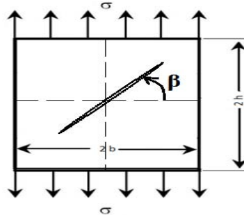
Figure 5: Cracked plate specimens.
