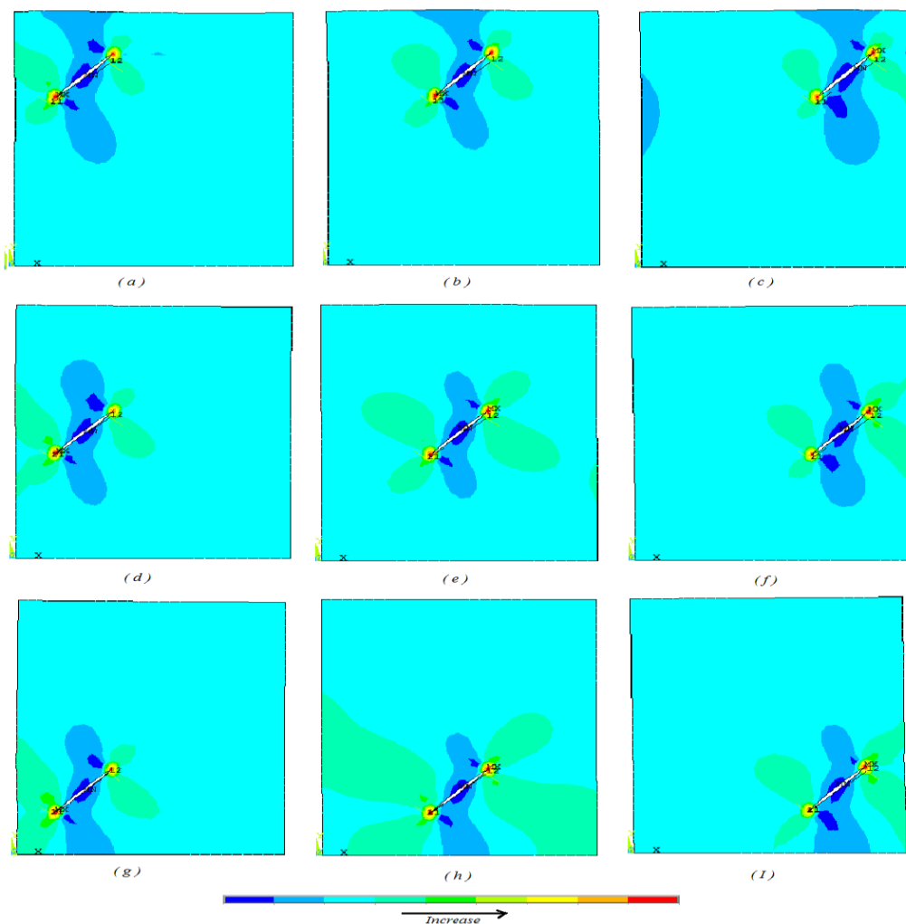
Figure 11: Contour plots of Von-Mises stress with the variation of crack location at \beta = 45^\circ .
