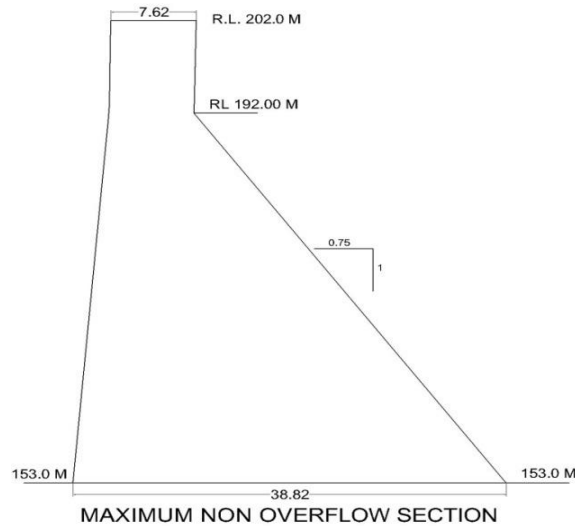
Figure 1: Cross Sections of Omkareshwar Dam from DPR
