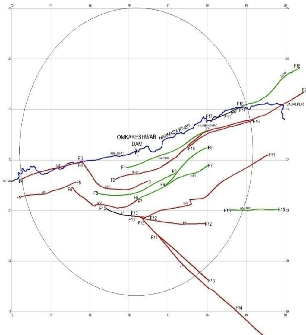
Figure 2: Fault map for SHA prepared from Seismotectonic Atlas of India for Omkareshwar Dam
