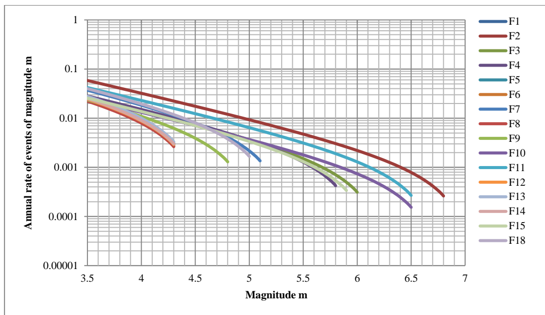
Figure 4: Fault level recurrence relation
