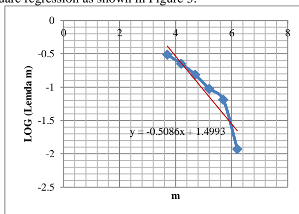
Figure 3: Gutenberg Richter relationship
