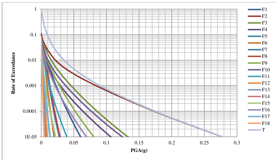
Figure 5: Seismic Hazard Curves for Omkareshwar Dam Site
