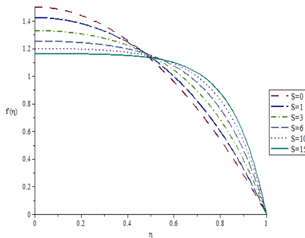
Figure 3: The influence of positive S on f(\eta) for two dimensional case
